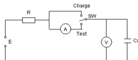
Measurement circuit 测试电路
